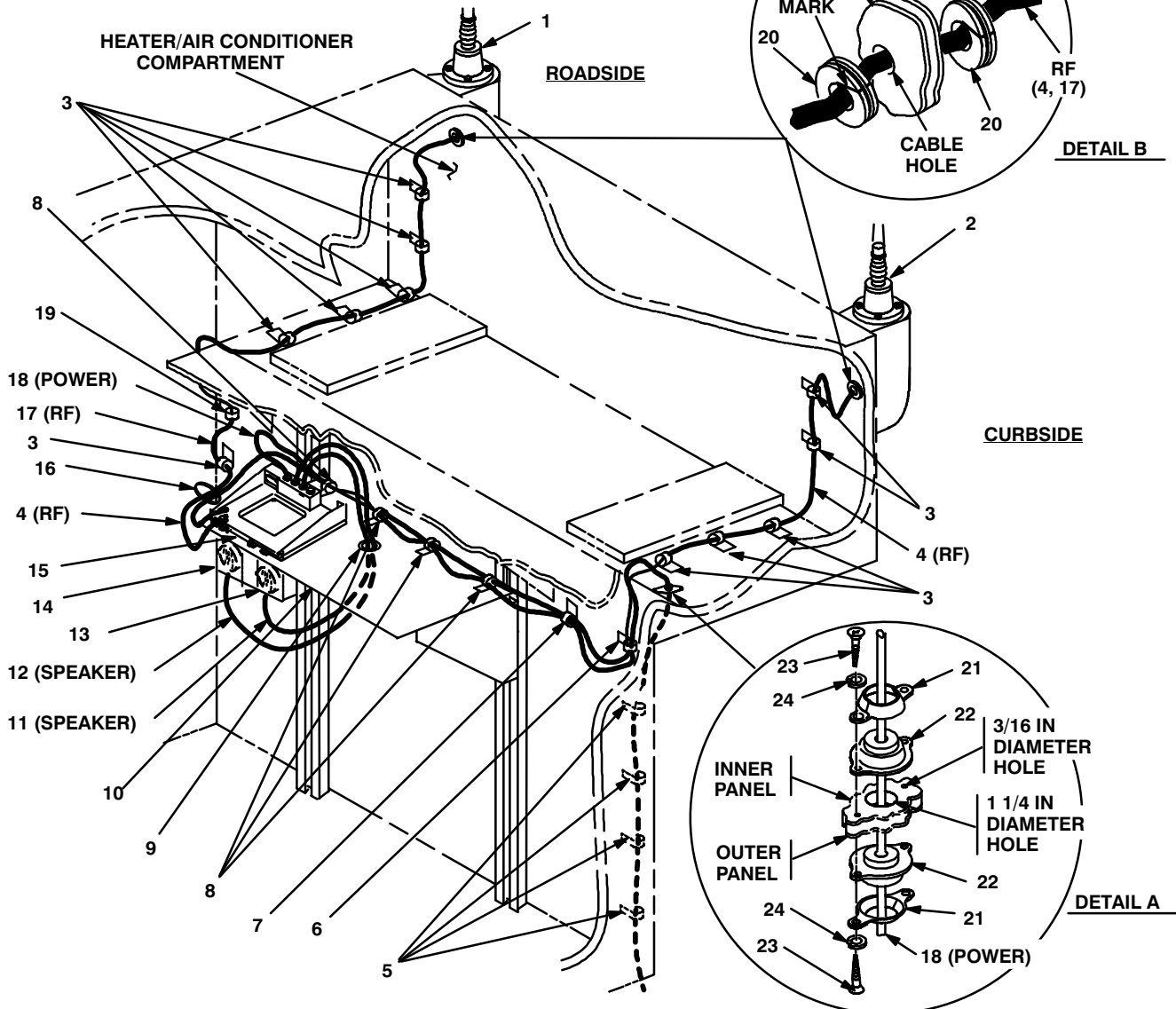
Figure 5-7 (1). Cable Installation: RF, Speaker and Power Cabling
