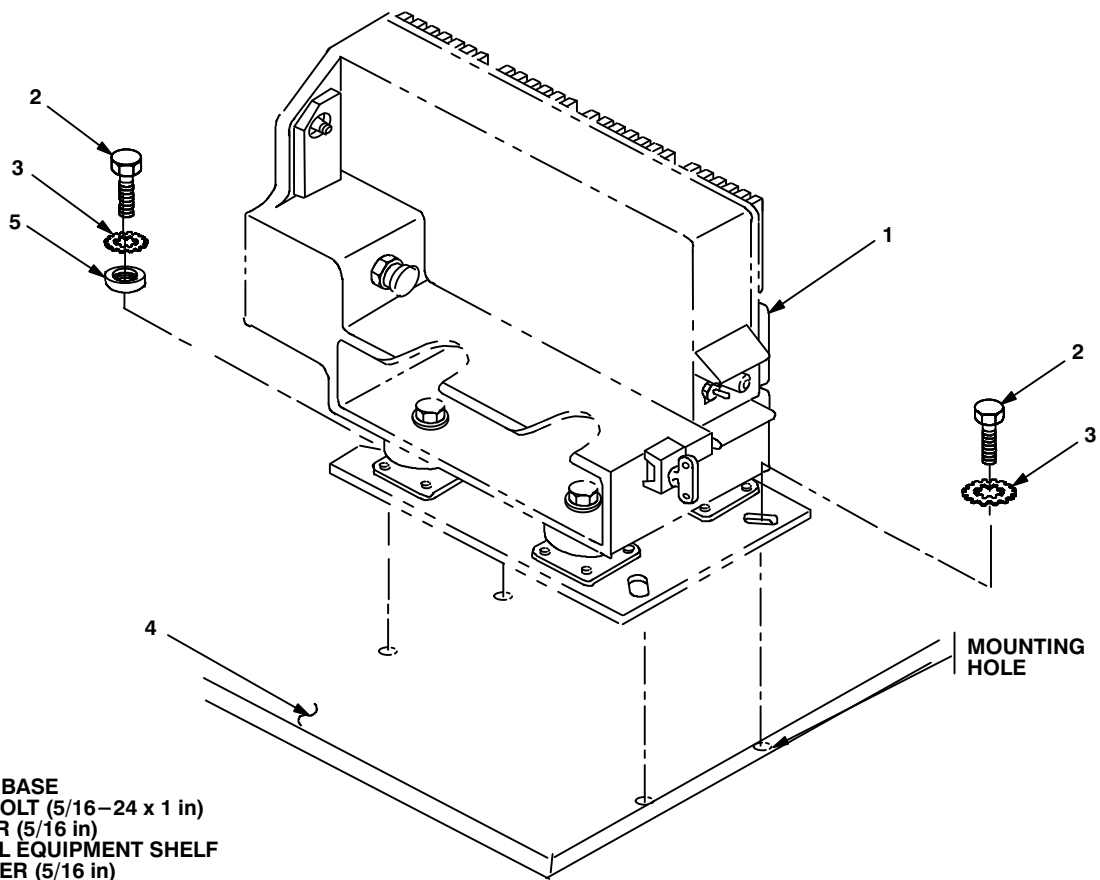
Figure 5-8. MT-6353/VRC Mounting Base Installation
