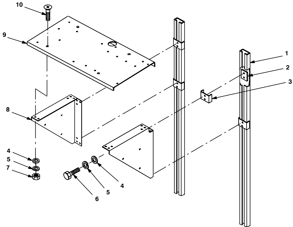
Figure 5-4 (2). Electrical Equipment Shelf Installation: Alternate Installation A
